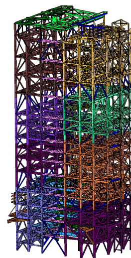
Figure 9: Analysis Model for TSL Furnace Building
