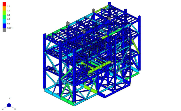
Figure 10: Member Capacity Utilisation Ratios for a Module
