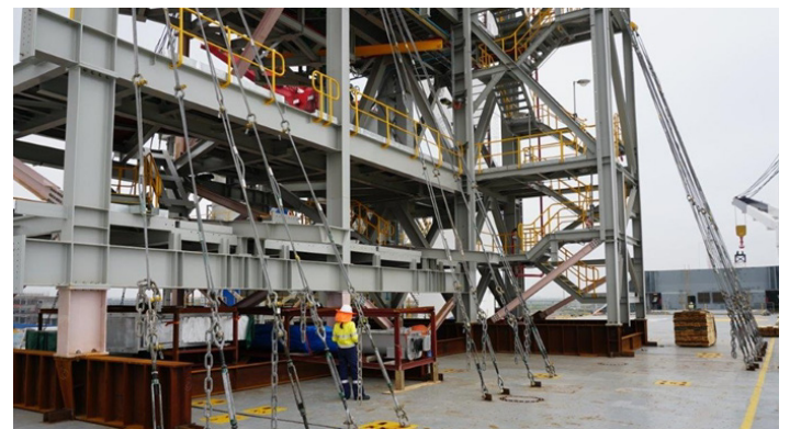
Figure 5: Module Lashed to Ship Deck
