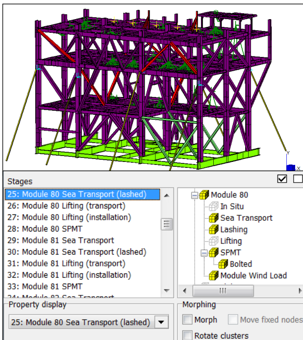
Figure 11: Analysis Stage –Sea Transport of a Module
